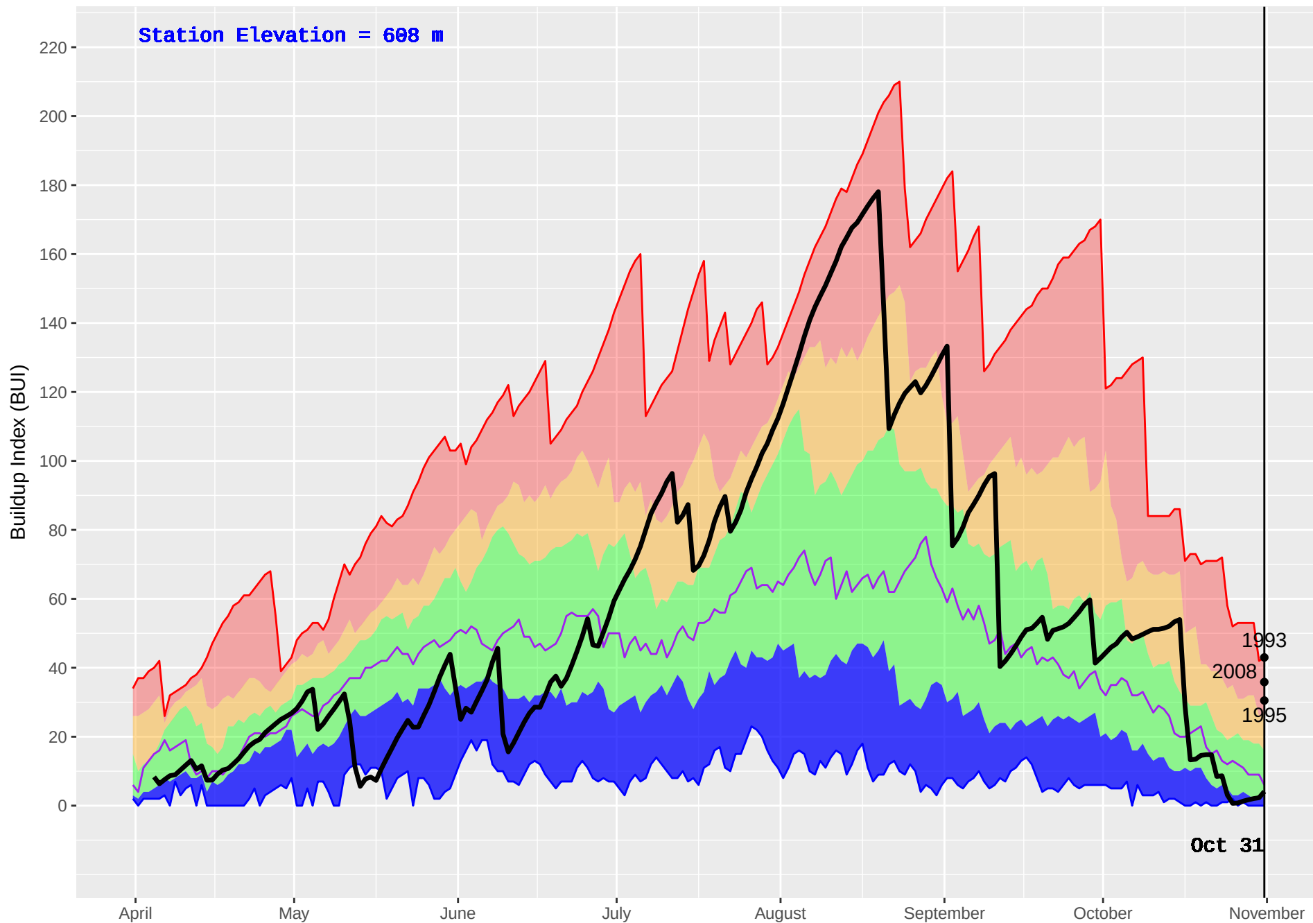
HOUSTON(DUNGATE) (162) : Historical (1974–2016) and Current (2017) Noon Buildup Index (BUI)
