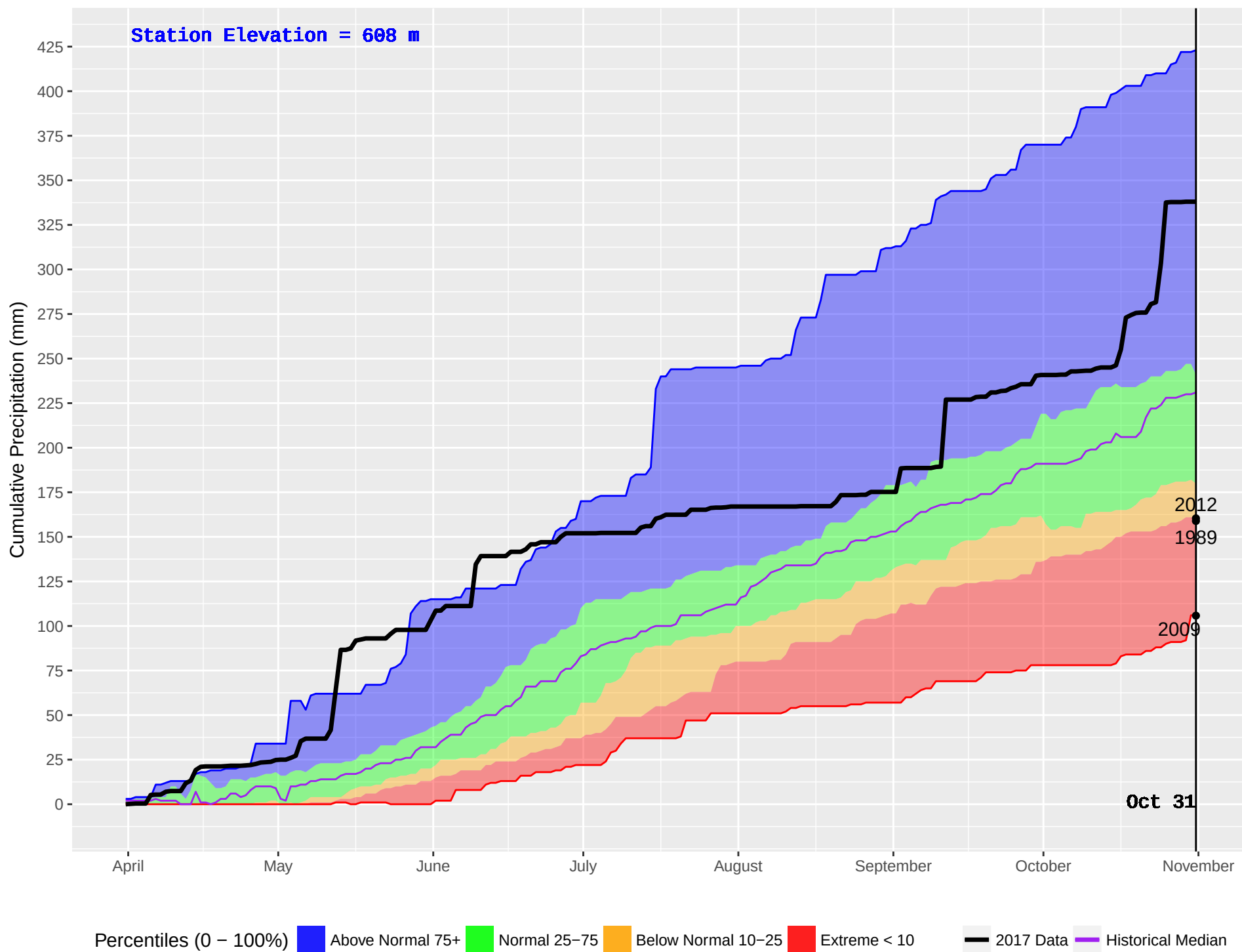
HOUSTON(DUNGATE) (162) : Historical (1974–2016) and Current (2017) Noon Cumulative Precipitation
